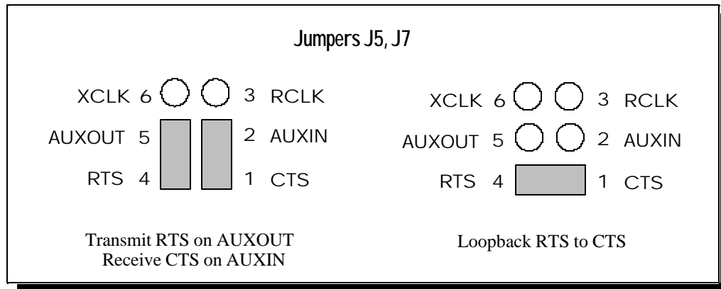
Figure 19 --- RTS/CTS selection
